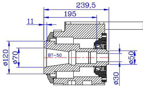
X-X View (Spindle Hole)
