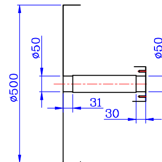
Spindle Hole
