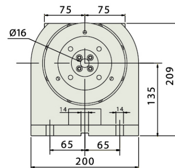
FT-135PD 圓盤尾座及氣壓延遲閥 FT-135PD Faceplate tailstock and air pneumatic delay valve
